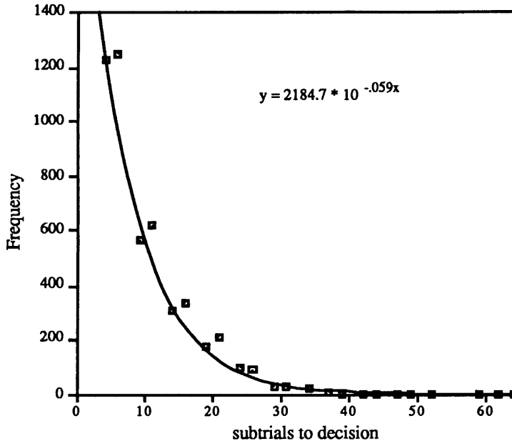
Figure 3 Exponential curve fit to Monte Carlo Results
